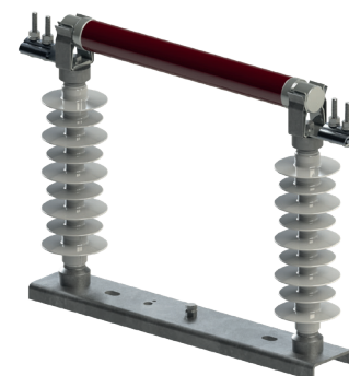
PBNWMA-30/50S izolatory silikonowe
